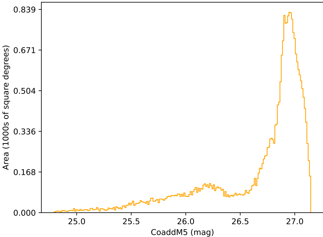
internal_u_expt60_nscale1.5v3.4_10yrs All sky r band: CoaddM5
