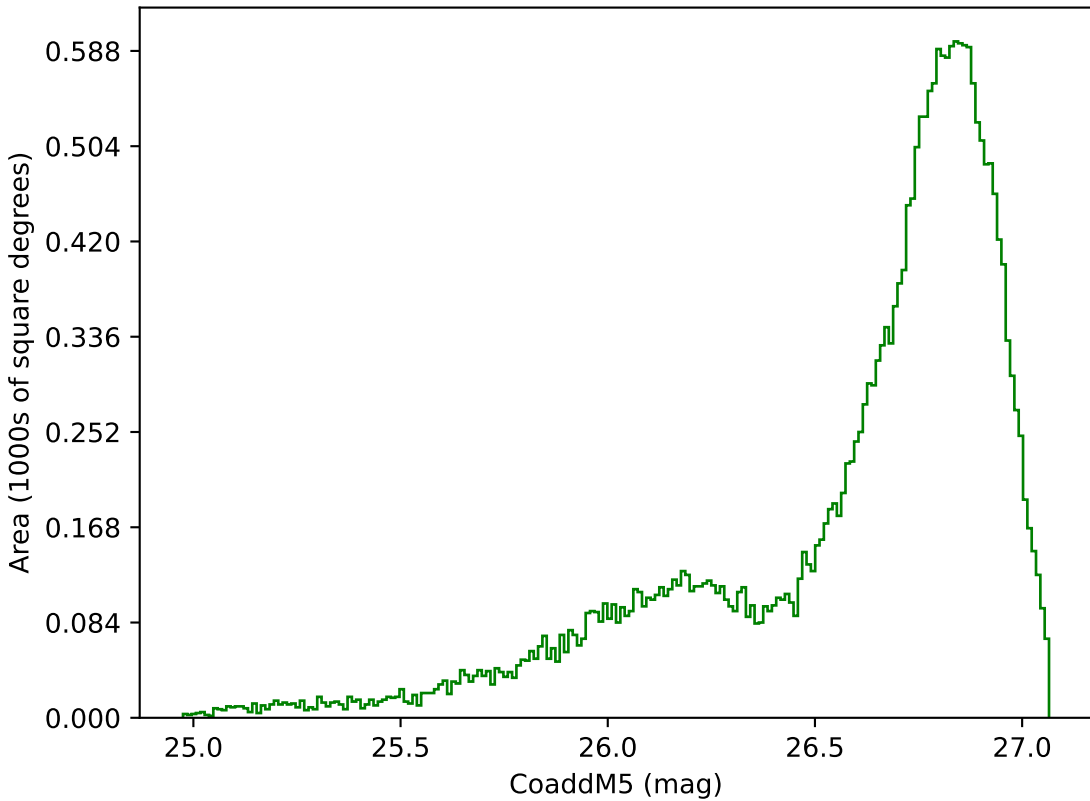
internal_u_expt60_nscale1.5v3.4_10yrs All sky g band: CoaddM5
