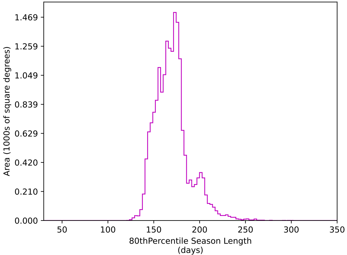
internal_u_expt60_nscale1.5v3.4_10yrs WFD z band: 80thPercentile Season Length
