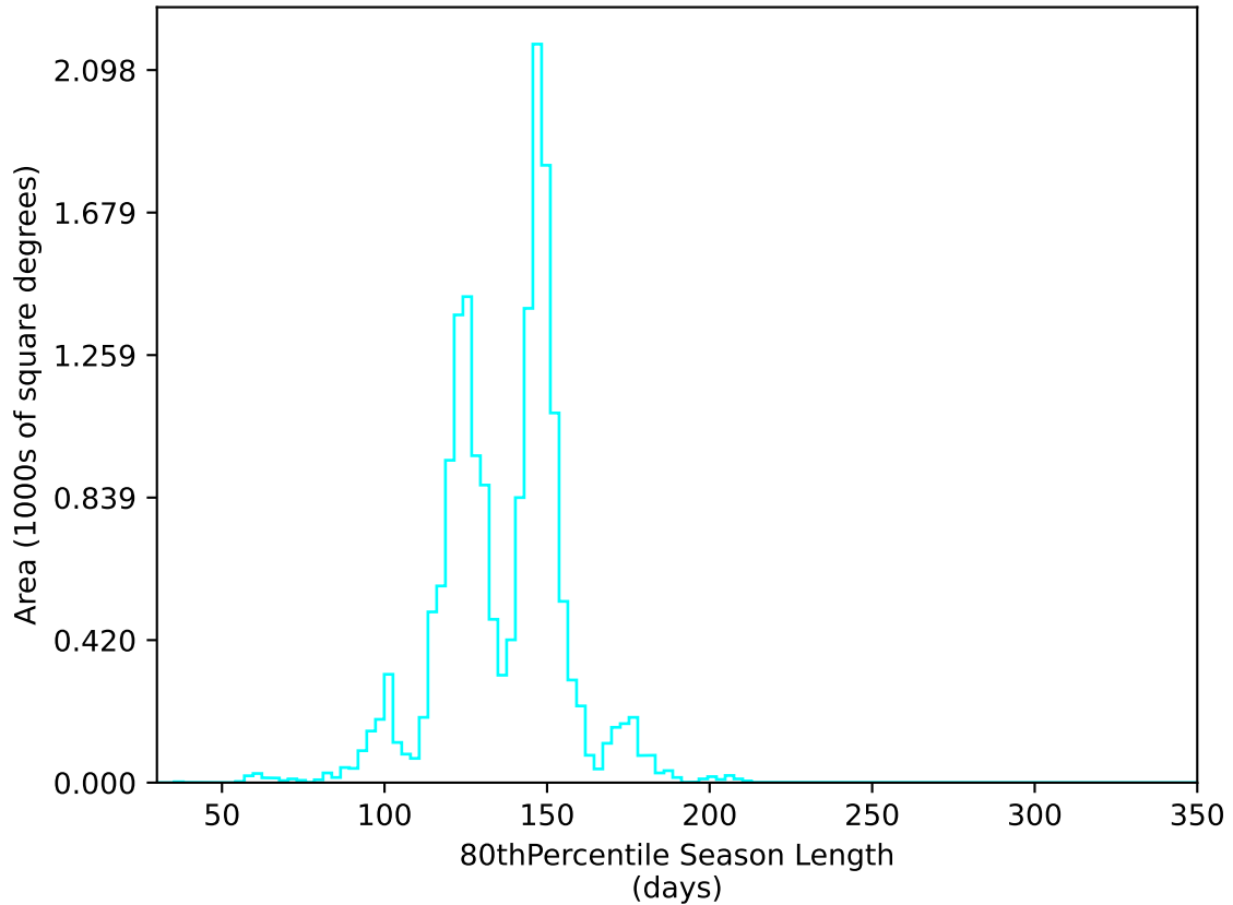
internal_u_expt60_nscale1.5v3.4_10yrs WFD u band: 80thPercentile Season Length
