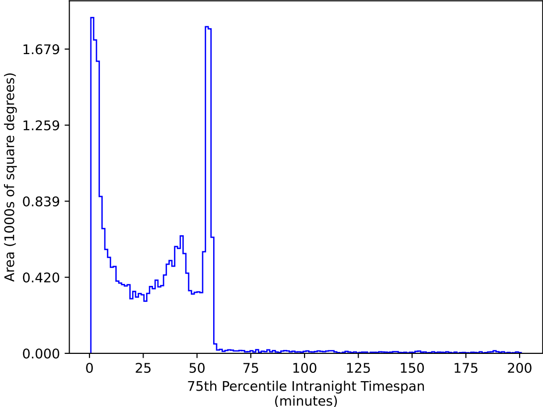
internal_u_expt60_nscale1.5v3.4_10yrs All sky ug bands: 75th Percentile Intranight Timespan
