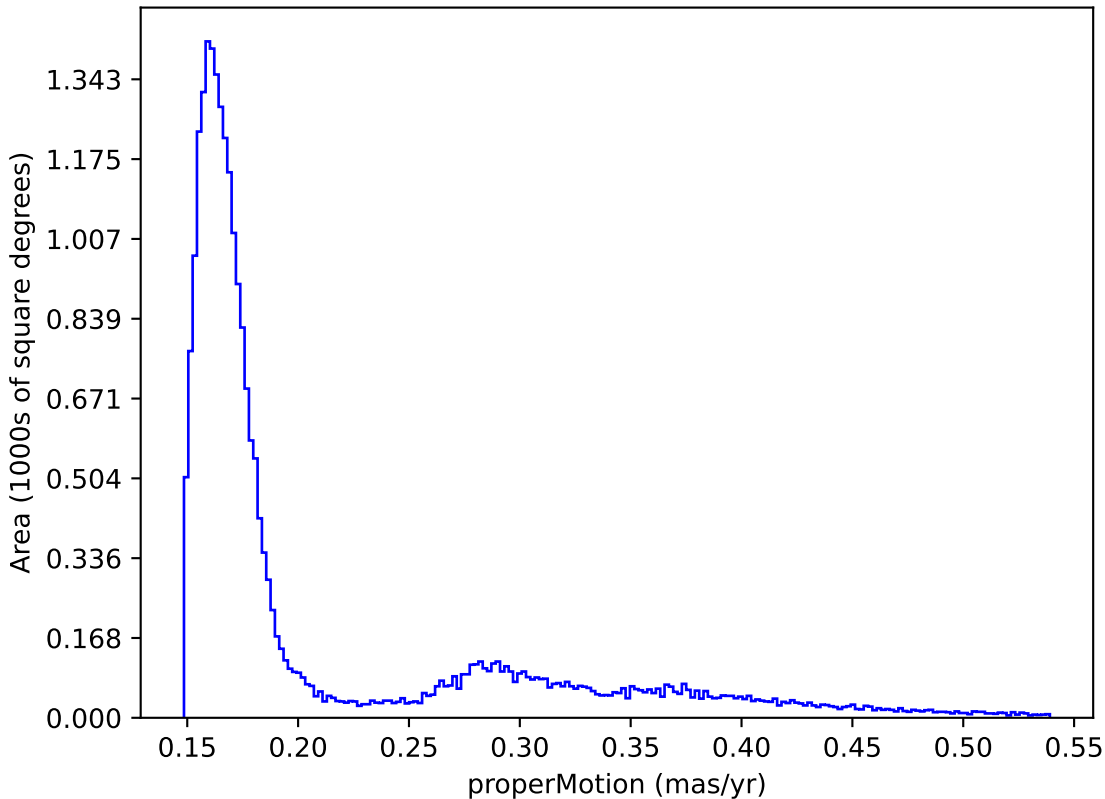
internal_u_expt60_nscale1.5v3.4_10yrs : properMotion
