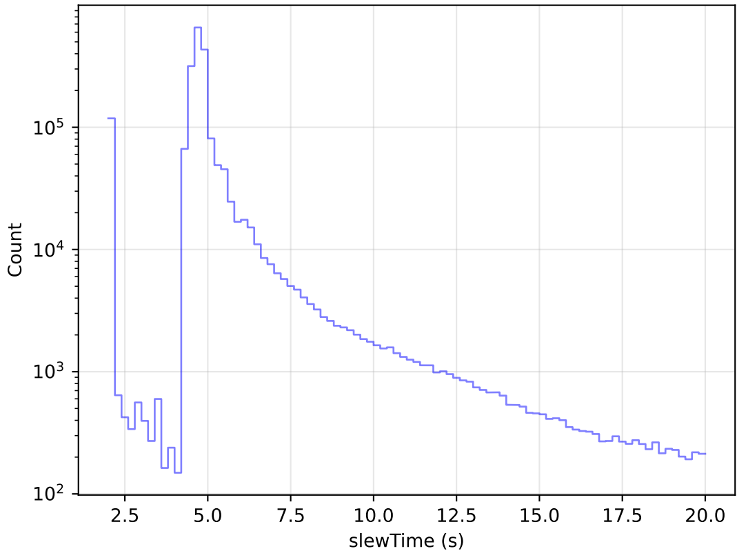
internal_u_expt60_nscale1.5v3.4_10yrs All visits: Zoom Slew Time Histogram
