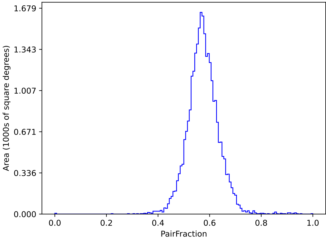
internal_u_expt60_nscale1.5v3.4_10yrs (g or r or i): PairFraction
