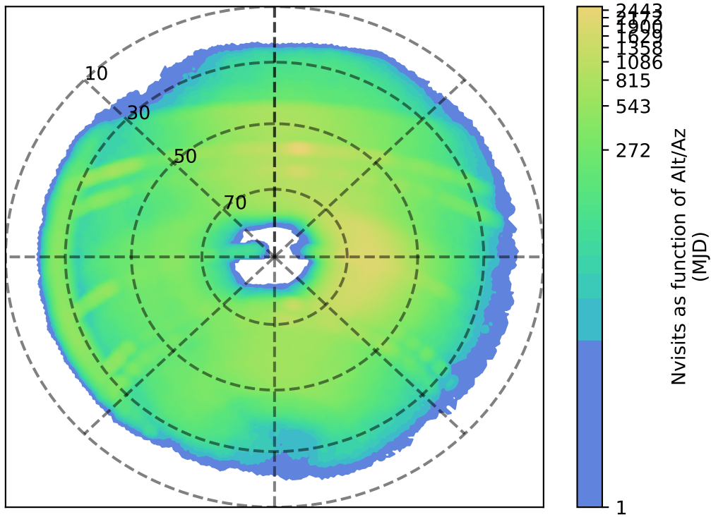
internal_u_expt60_nscale1.5v3.4_10yrs r: Nvisits as function of Alt/Az
