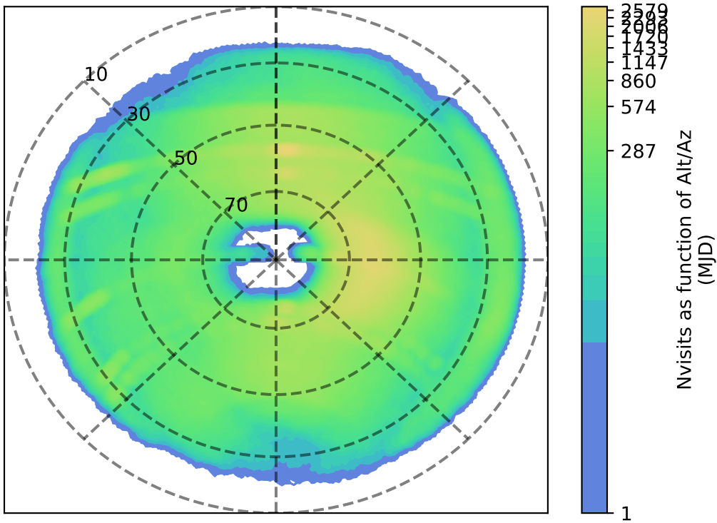
internal_u_expt60_nscale1.5v3.4_10yrs i: Nvisits as function of Alt/Az
