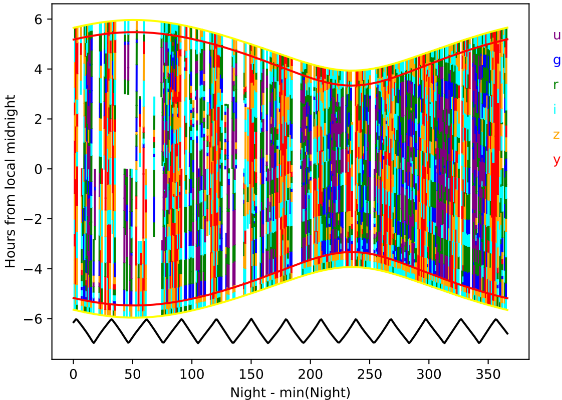
internal_u_expt60_nscale1.5v3.4_10yrs year 9-10: Hourglass
