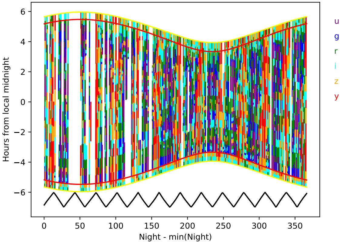
internal_u_expt60_nscale1.5v3.4_10yrs year 8-9: Hourglass
