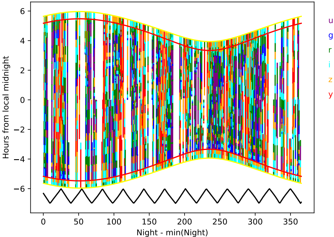
internal_u_expt60_nscale1.5v3.4_10yrs year 7-8: Hourglass
