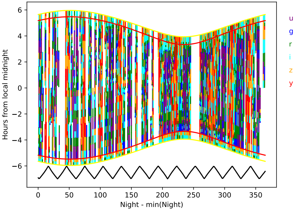
internal_u_expt60_nscale1.5v3.4_10yrs year 5-6: Hourglass
