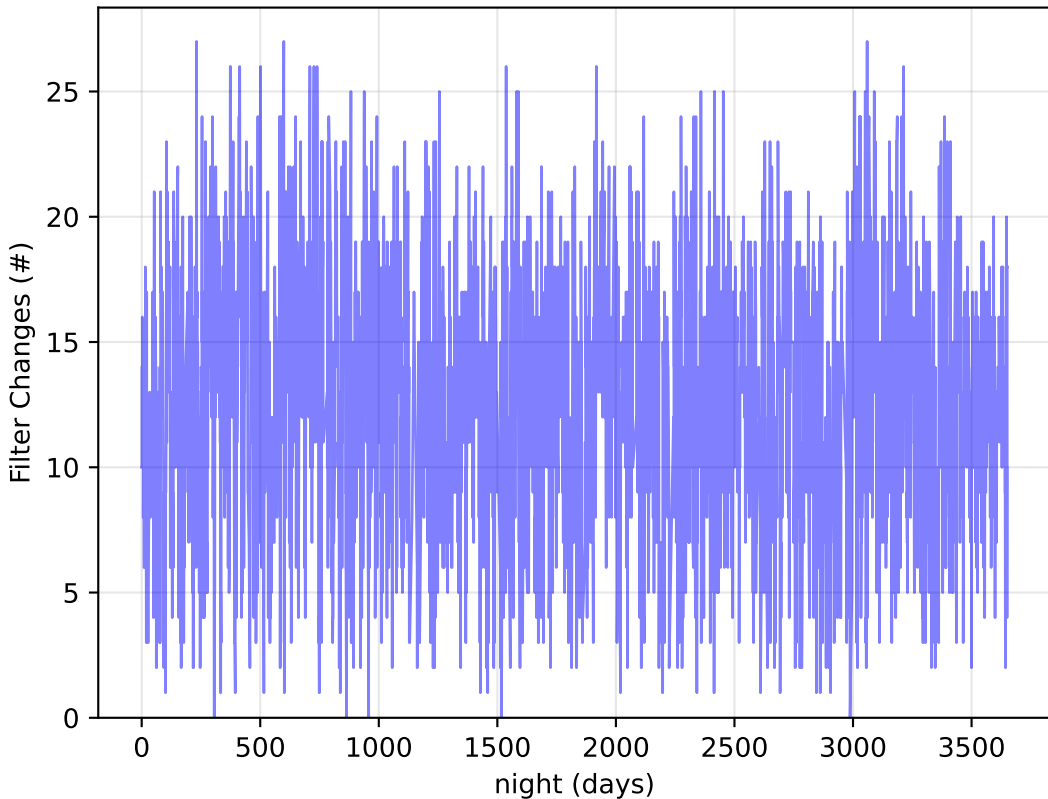
internal_u_expt60_nscale1.5v3.4_10yrs : Filter Changes
