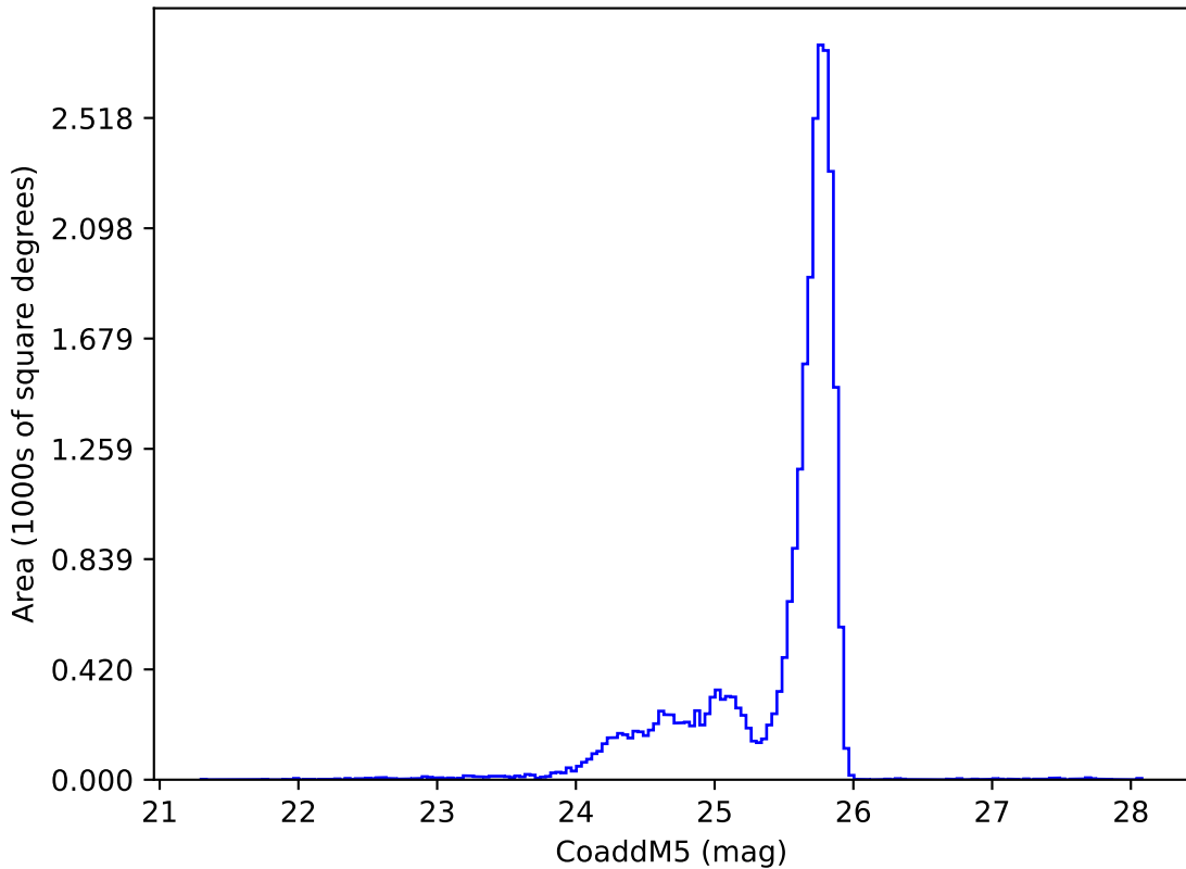
internal_u_expt60_nscale1.5v3.4_10yrs z: CoaddM5
