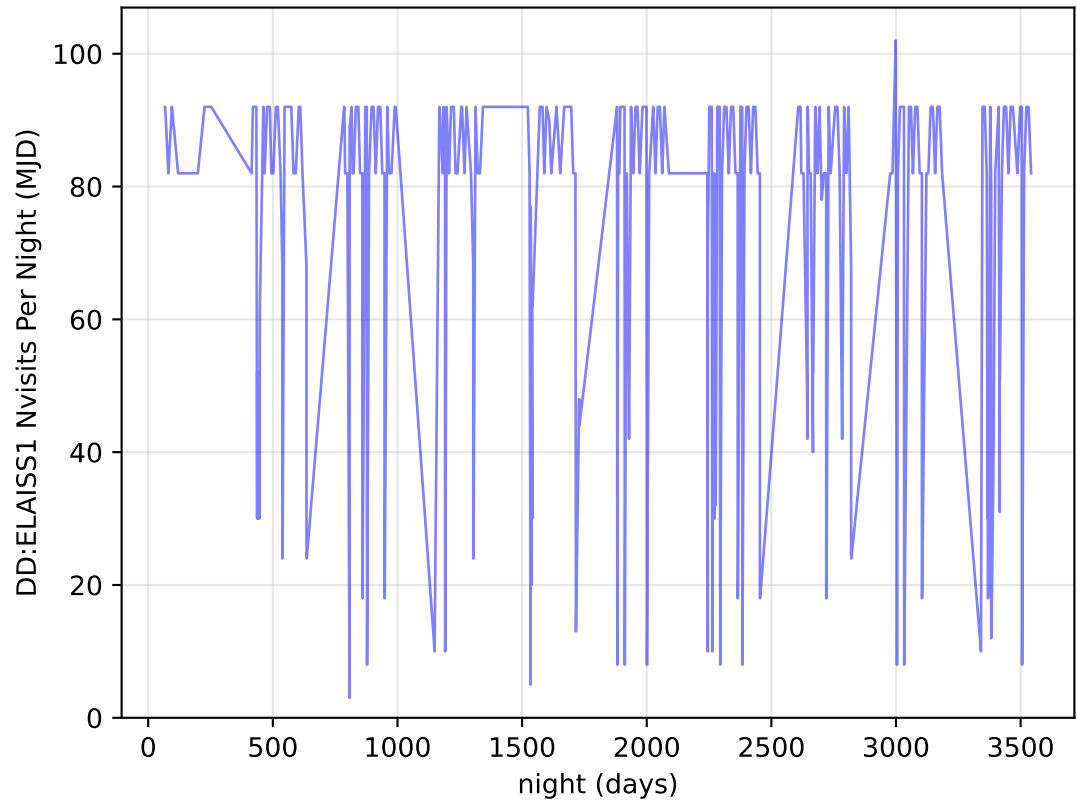
internal_u_expt60_nscale1.5v3.4_10yrs all bands: DD:ELAISS1 Nvisits Per Night
