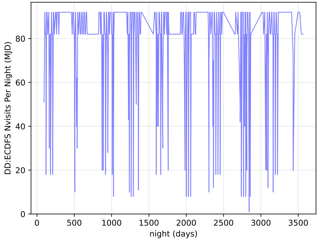
internal_u_expt60_nscale1.5v3.4_10yrs all bands: DD:ECDFS Nvisits Per Night
