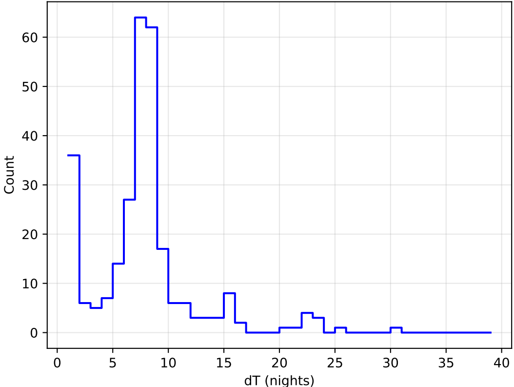
internal_u_expt60_nscale1.5v3.4_10yrs all bands: DD:ECDFS Delta Nights Histogram
