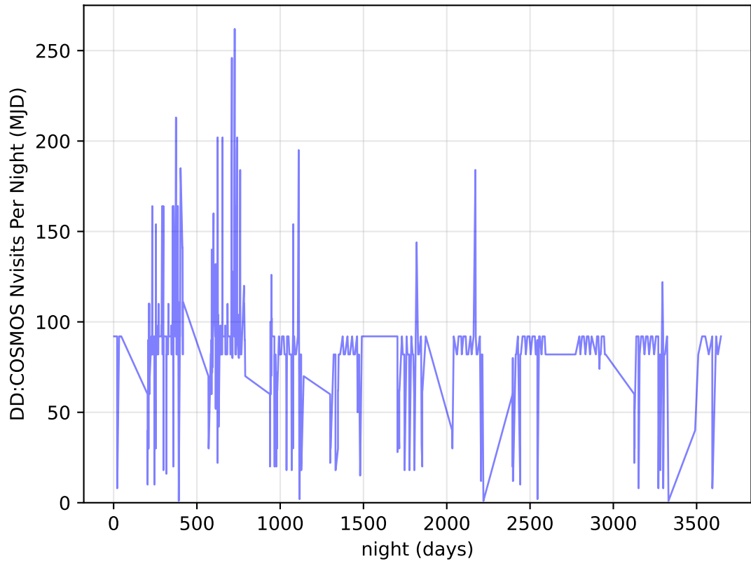
internal_u_expt60_nscale1.5v3.4_10yrs all bands: DD: COSMOS Nvisits Per Night
