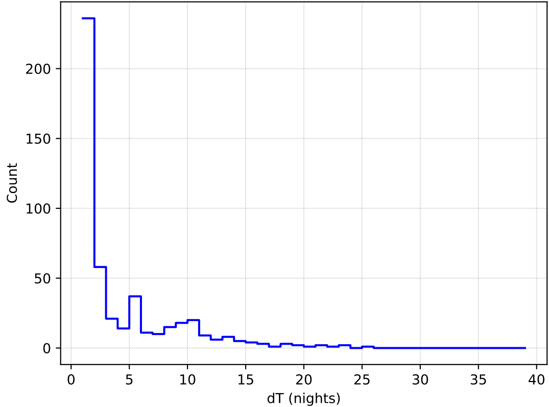
internal_u_expt60_nscale1.5v3.4_10yrs all bands: DD: COSMOS Delta Nights Histogram
