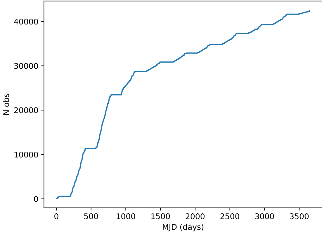
internal_u_expt60_nscale1.5v3.4_10yrs all bands: DD: COSMOS Cumulative NVisits
