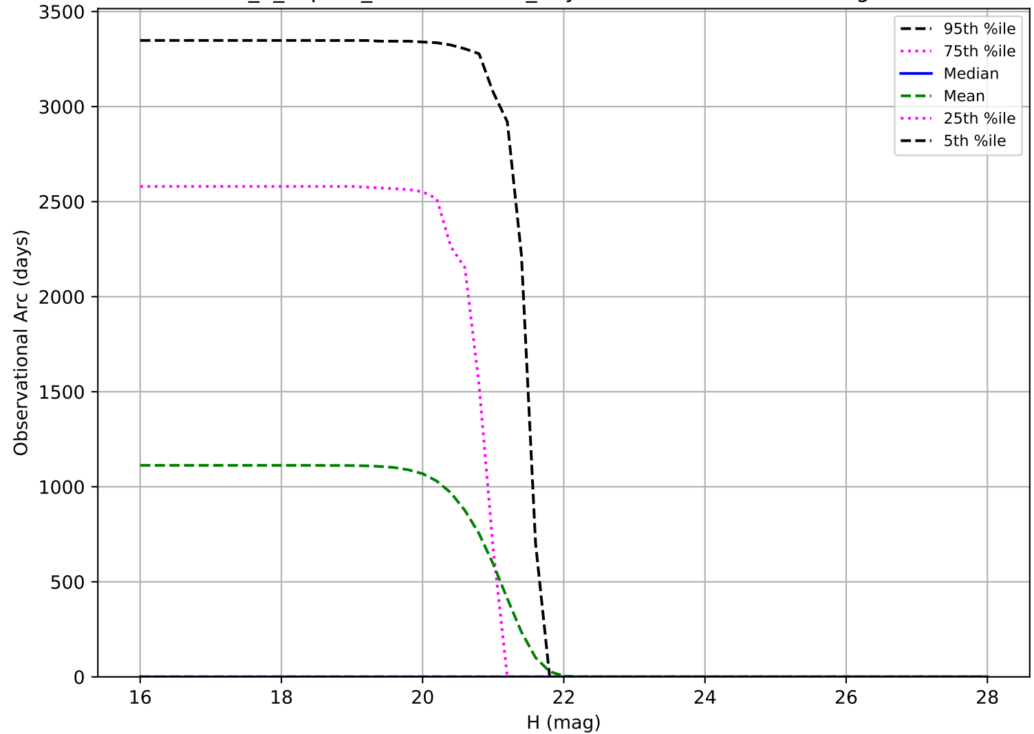
internal_u_expt60_nscale1.2v3.4_10yrs: Observational Arc Length Vatra
