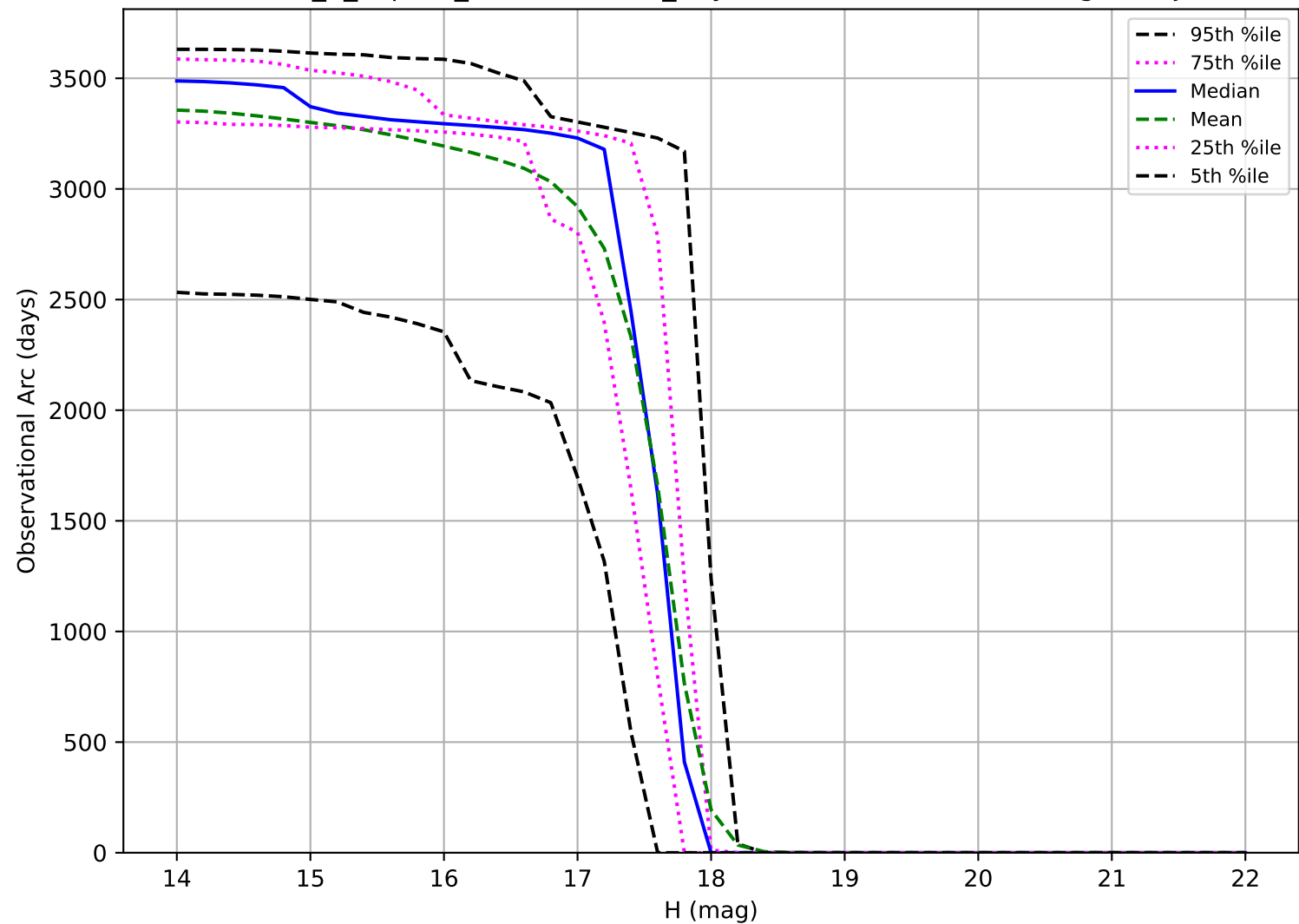
internal_u_expt60_nscale1.2v3.4_10yrs: Observational Arc Length Trojan
