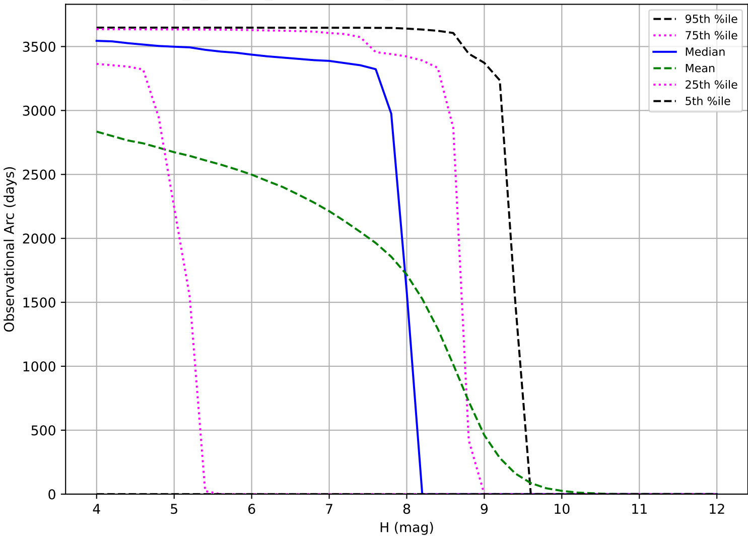
internal_u_expt60_nscale1.2v3.4_10yrs: Observational Arc Length TNO
