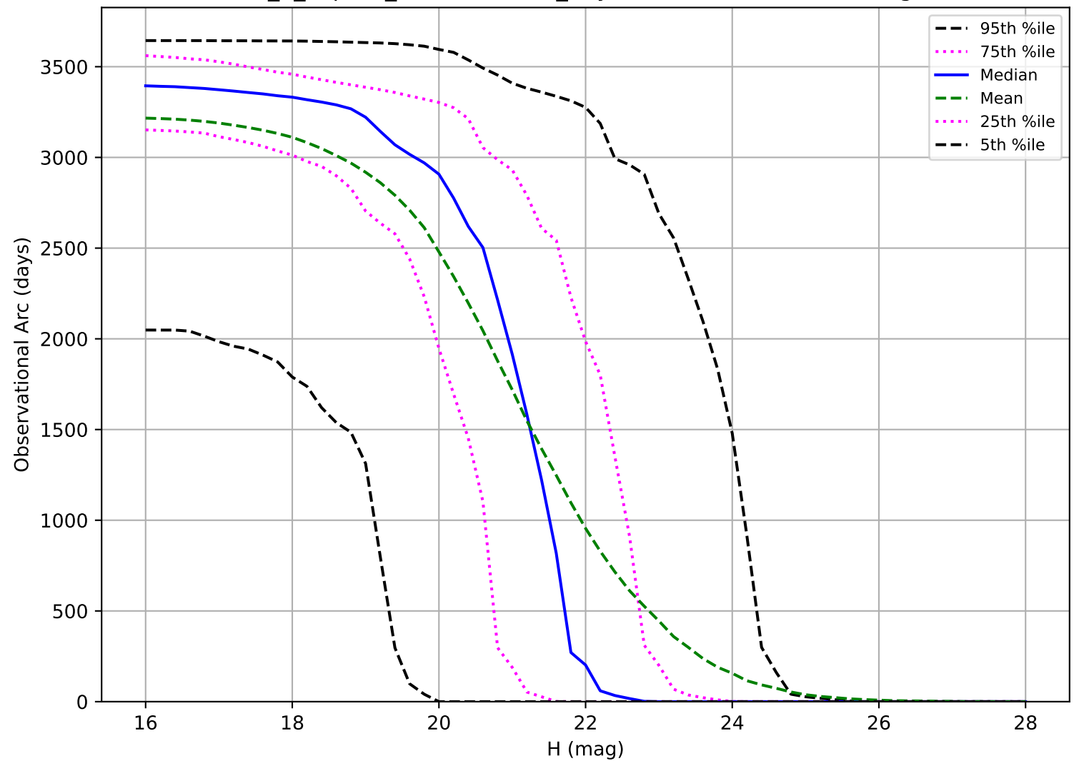
internal_u_expt60_nscale1.2v3.4_10yrs: Observational Arc Length PHA
