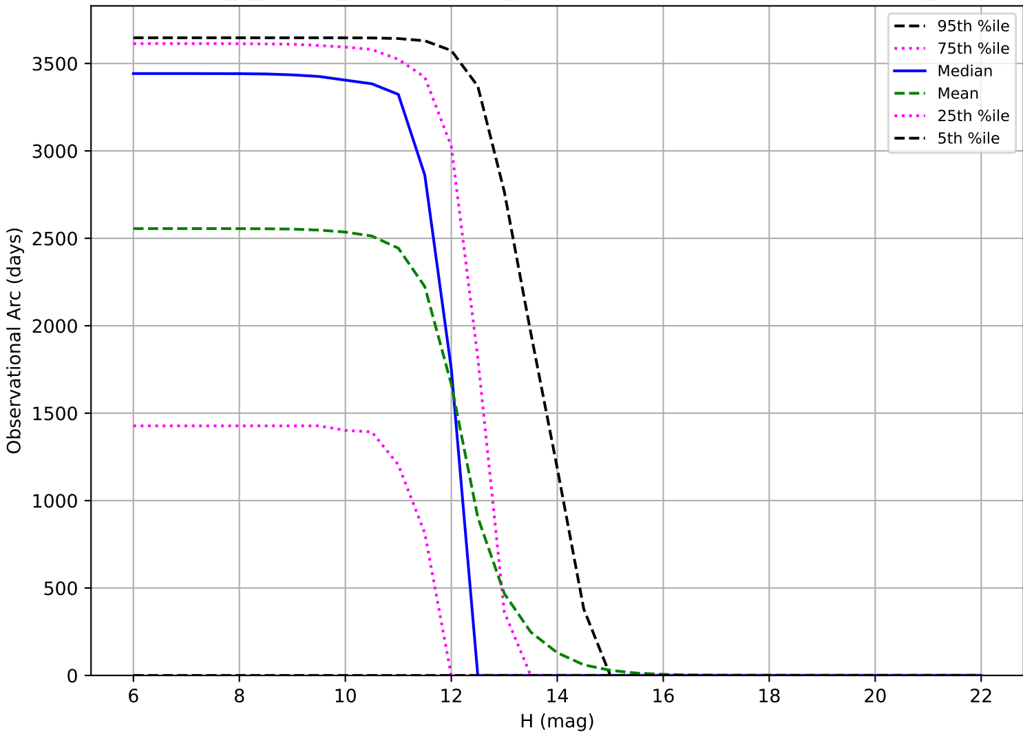
internal_u_expt60_nscale1.2v3.4_10yrs: Observational Arc Length OCC_r20
