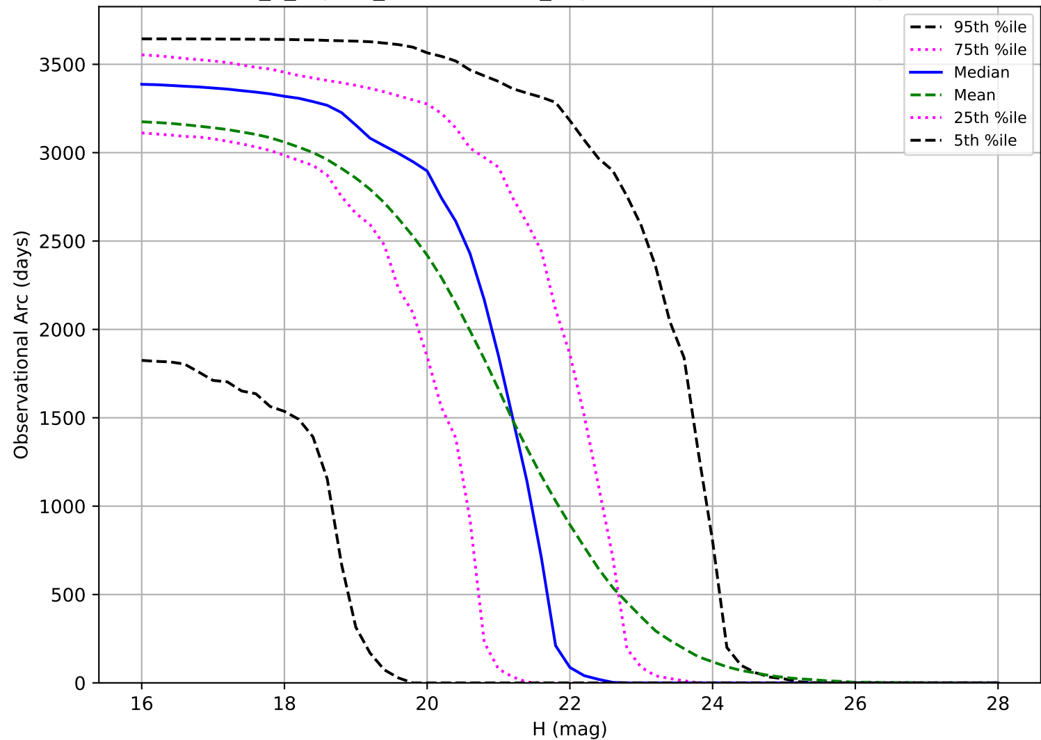
internal_u_expt60_nscale1.2v3.4_10yrs: Observational Arc Length NEO
