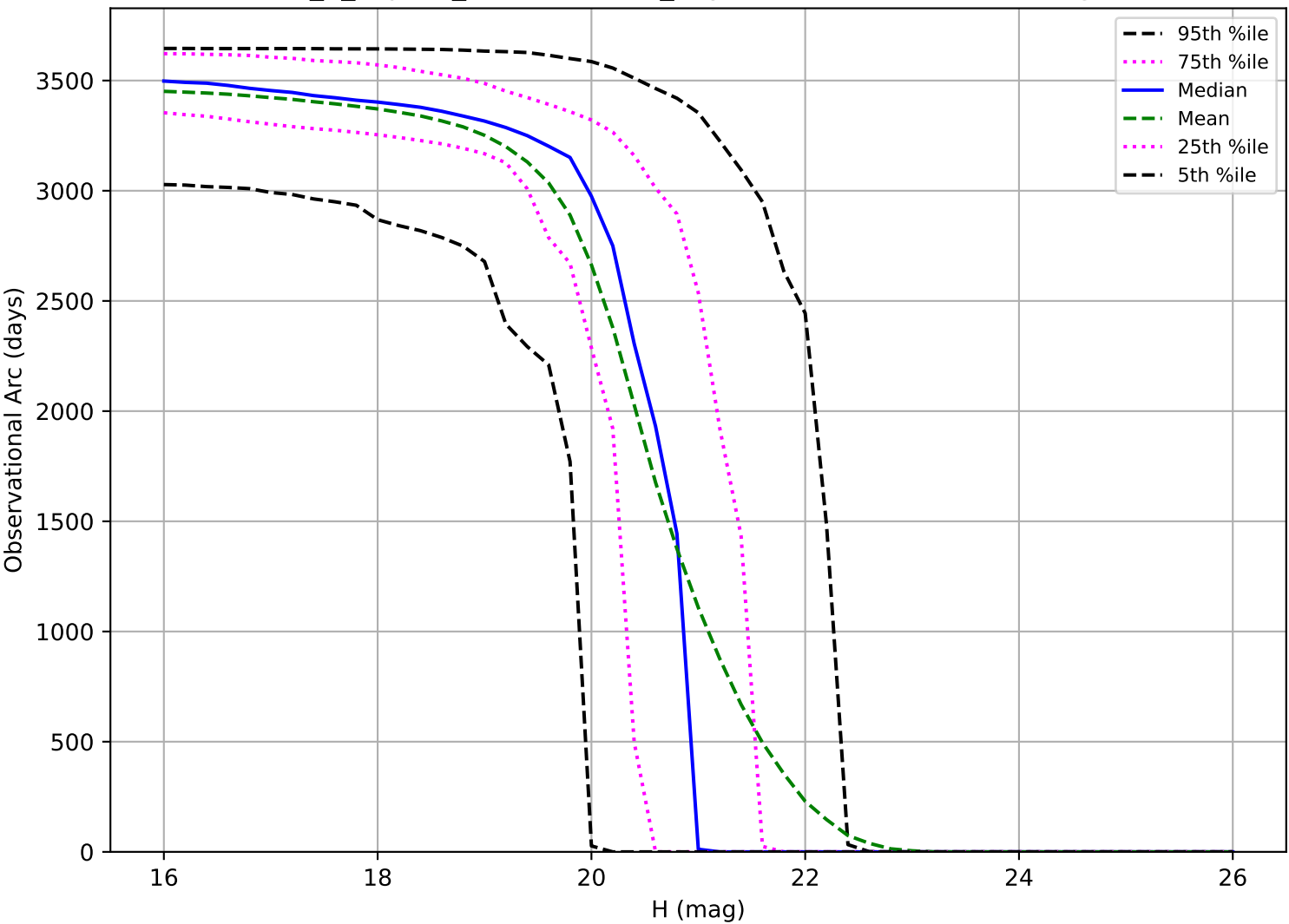
internal_u_expt60_nscale1.2v3.4_10yrs: Observational Arc Length MBA
