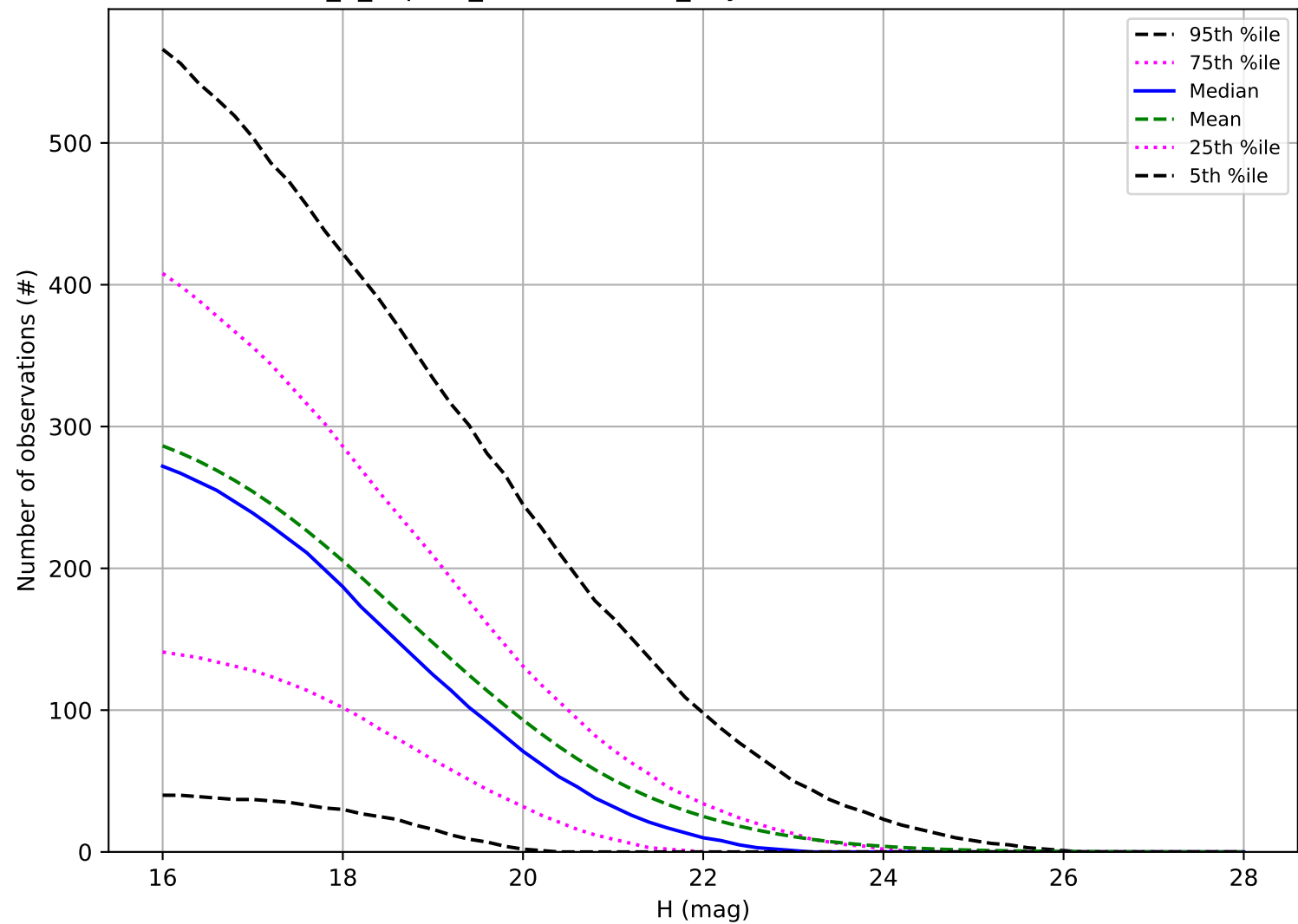
internal_u_expt60_nscale1.2v3.4_10yrs: Number of observations PHA
