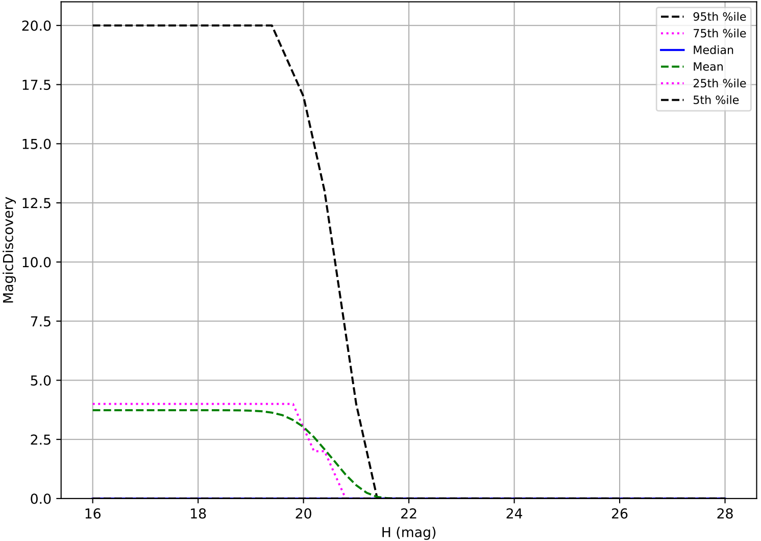
internal_u_expt60_nscale1.2v3.4_10yrs: Vatira 6 detections in 60 nights detection loss
