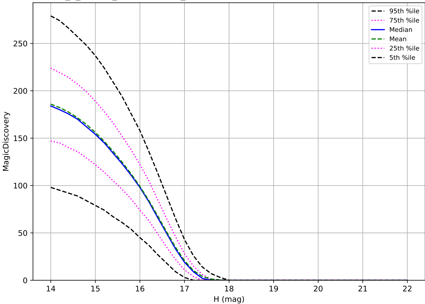
internal_u_expt60_nscale1.2v3.4_10yrs: Trojan 6 detections in 60 nights detection loss
