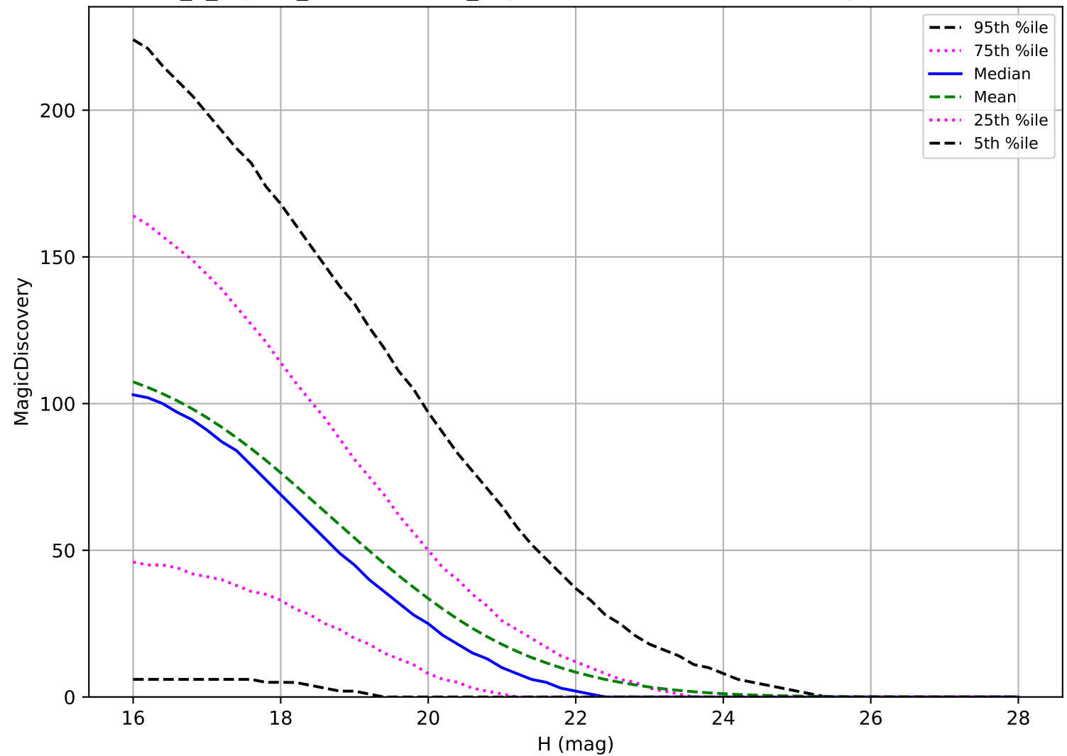
internal_u_expt60_nscale1.2v3.4_10yrs: PHA 6 detections in 60 nights detection loss
