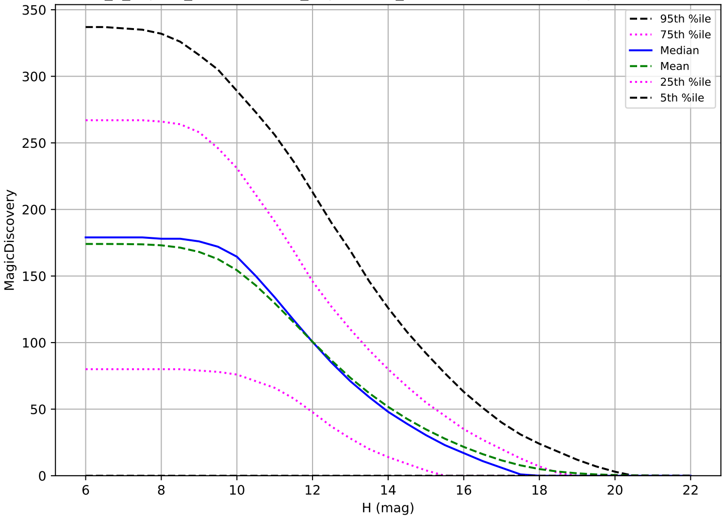
internal_u_expt60_nscale1.2v3.4_10yrs: OCC_r5 6 detections in 60 nights detection loss
