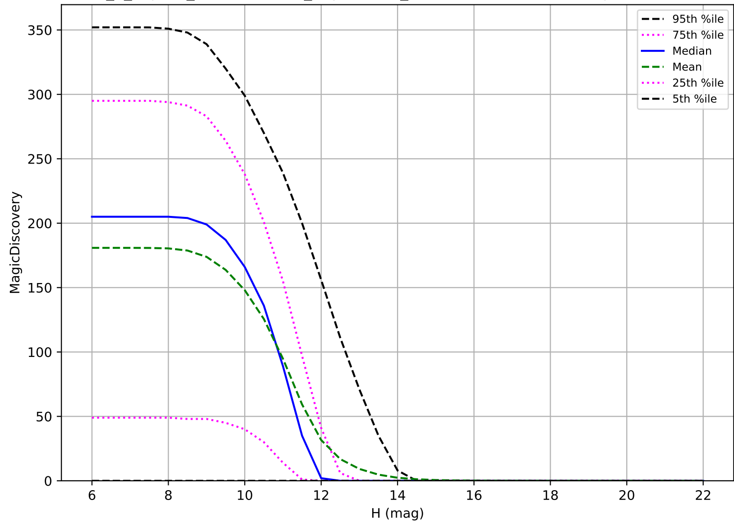
internal_u_expt60_nscale1.2v3.4_10yrs: OCC_r20 6 detections in 60 nights detection loss
