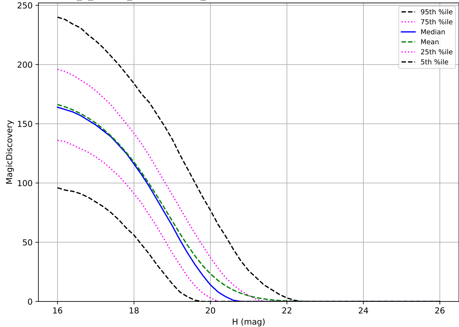
internal_u_expt60_nscale1.2v3.4_10yrs: MBA 6 detections in 60 nights detection loss
