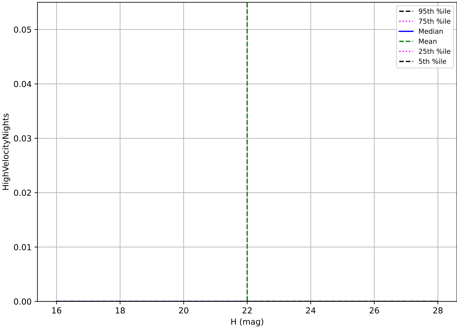
internal_u_expt60_nscale1.2v3.4_10yrs: Vatira High velocity pair detection loss
