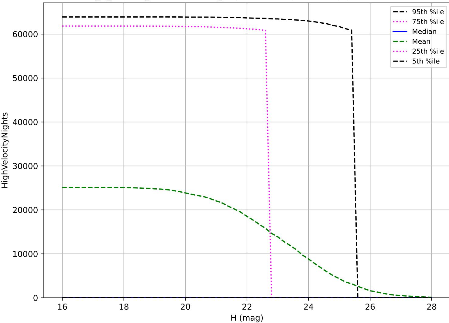
internal_u_expt60_nscale1.2v3.4_10yrs: PHA High velocity pair detection loss
