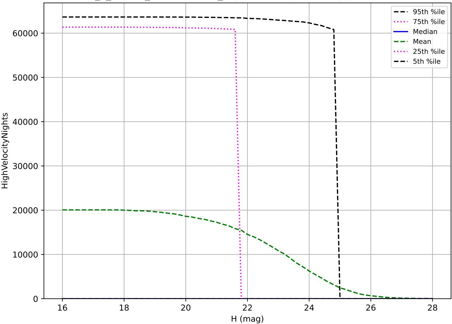
internal_u_expt60_nscale1.2v3.4_10yrs: NEO High velocity pair detection loss
