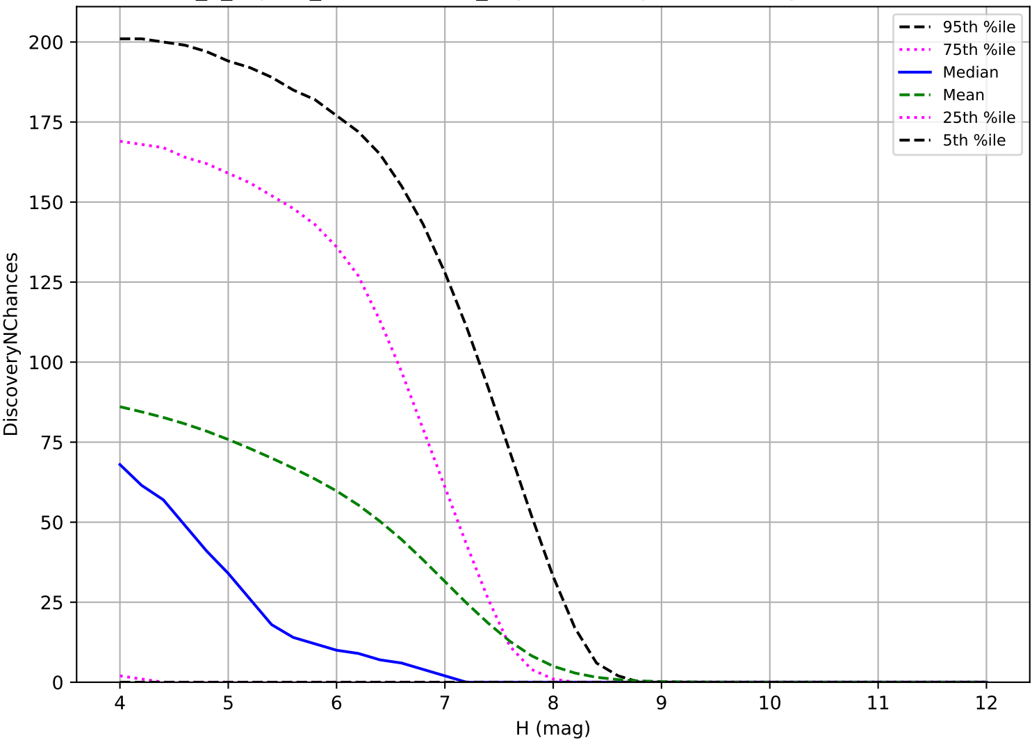
internal_u_expt60_nscale1.2v3.4_10yrs: TNO 3 pairs in 15 nights detection loss
