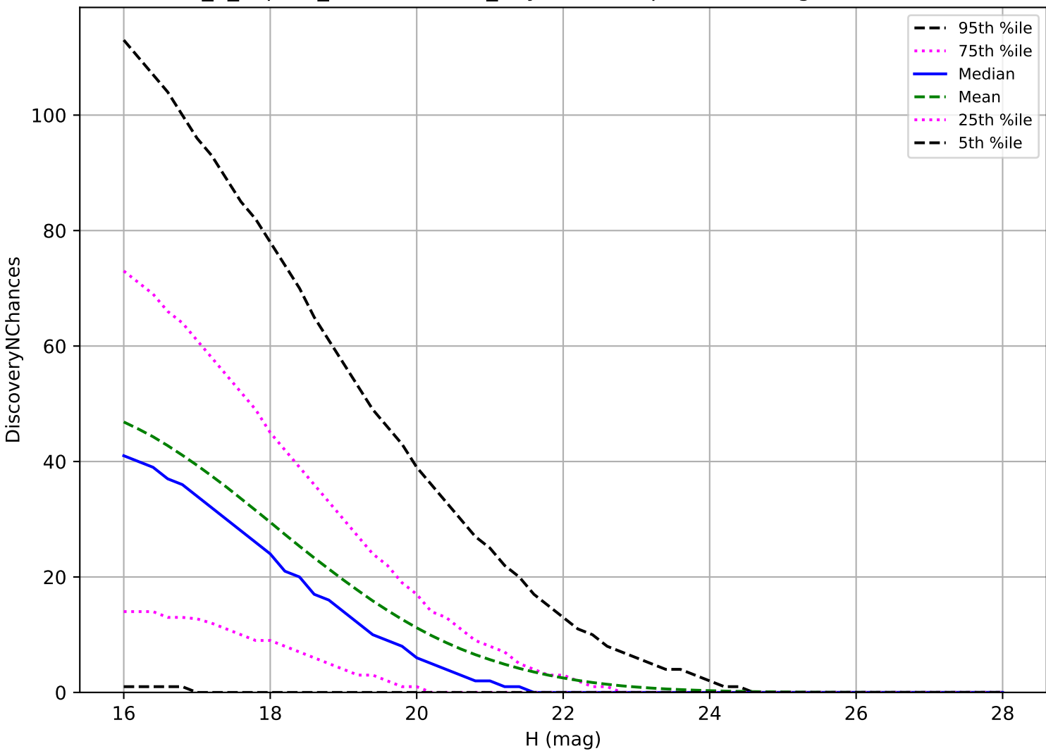
internal_u_expt60_nscale1.2v3.4_10yrs: PHA 3 pairs in 15 nights detection loss
