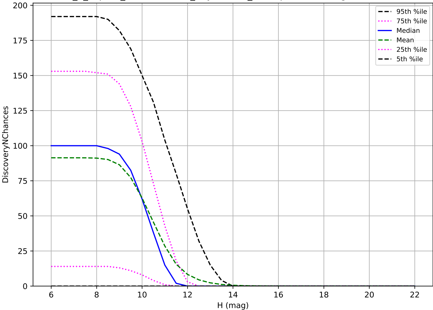
internal_u_expt60_nscale1.2v3.4_10yrs: OCC_r20 3 pairs in 15 nights detection loss
