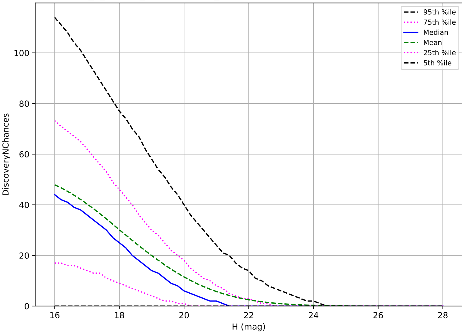
internal_u_expt60_nscale1.2v3.4_10yrs: NEO 3 pairs in 15 nights detection loss
