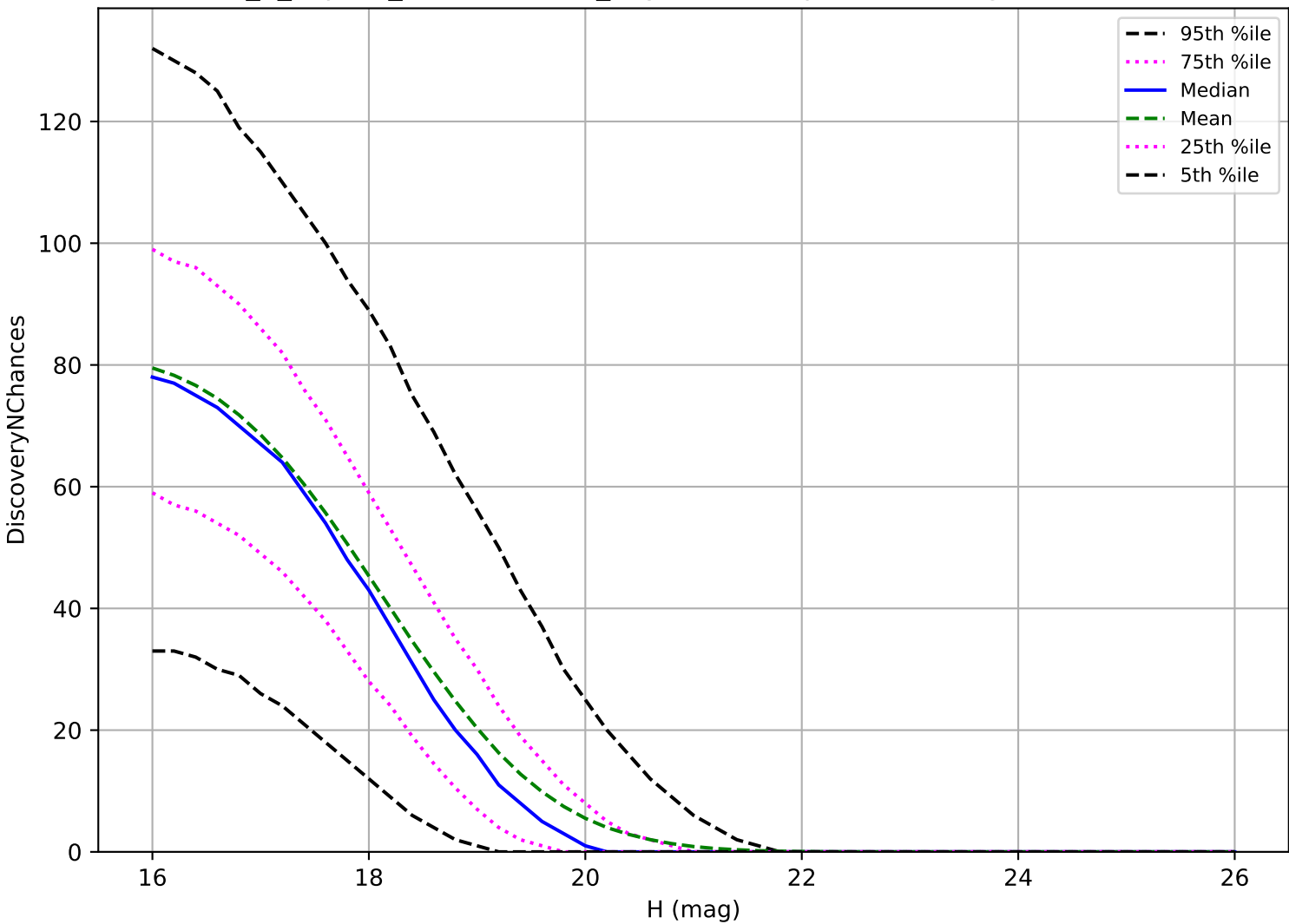
internal_u_expt60_nscale1.2v3.4_10yrs: MBA 3 pairs in 15 nights detection loss
