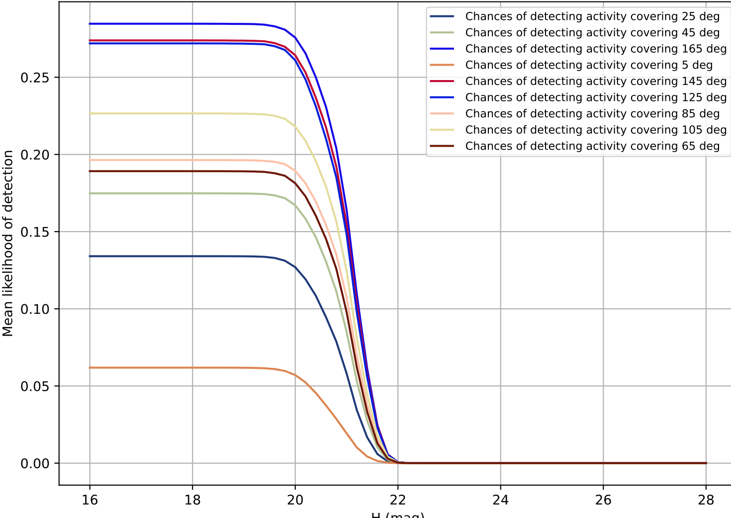
internal u expt60 nscale1.2v3.4 10yrs Vatira
