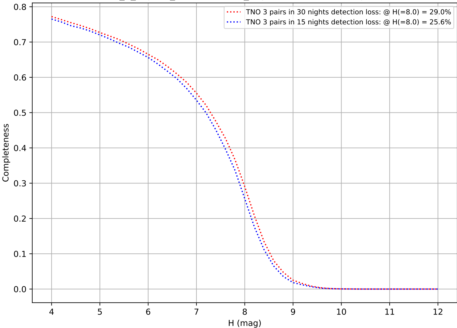
internal_u_expt60_nscale1.2v3.4_10yrs: DifferentialCompleteness
