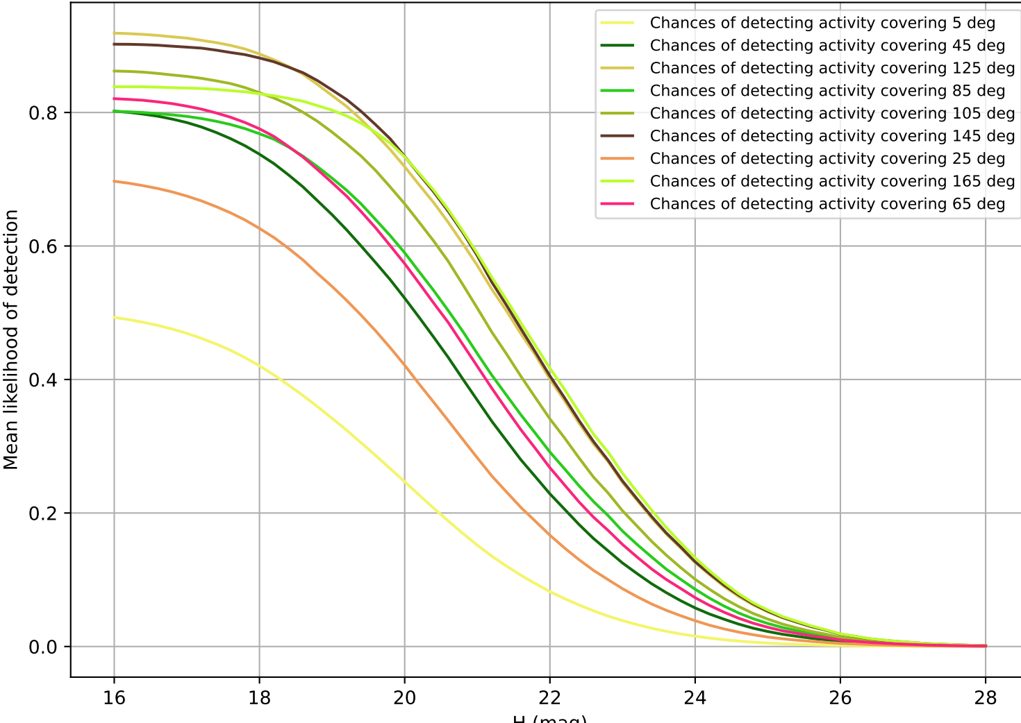
internal u expt60 nscale1.2v3.4 10yrs PHA
