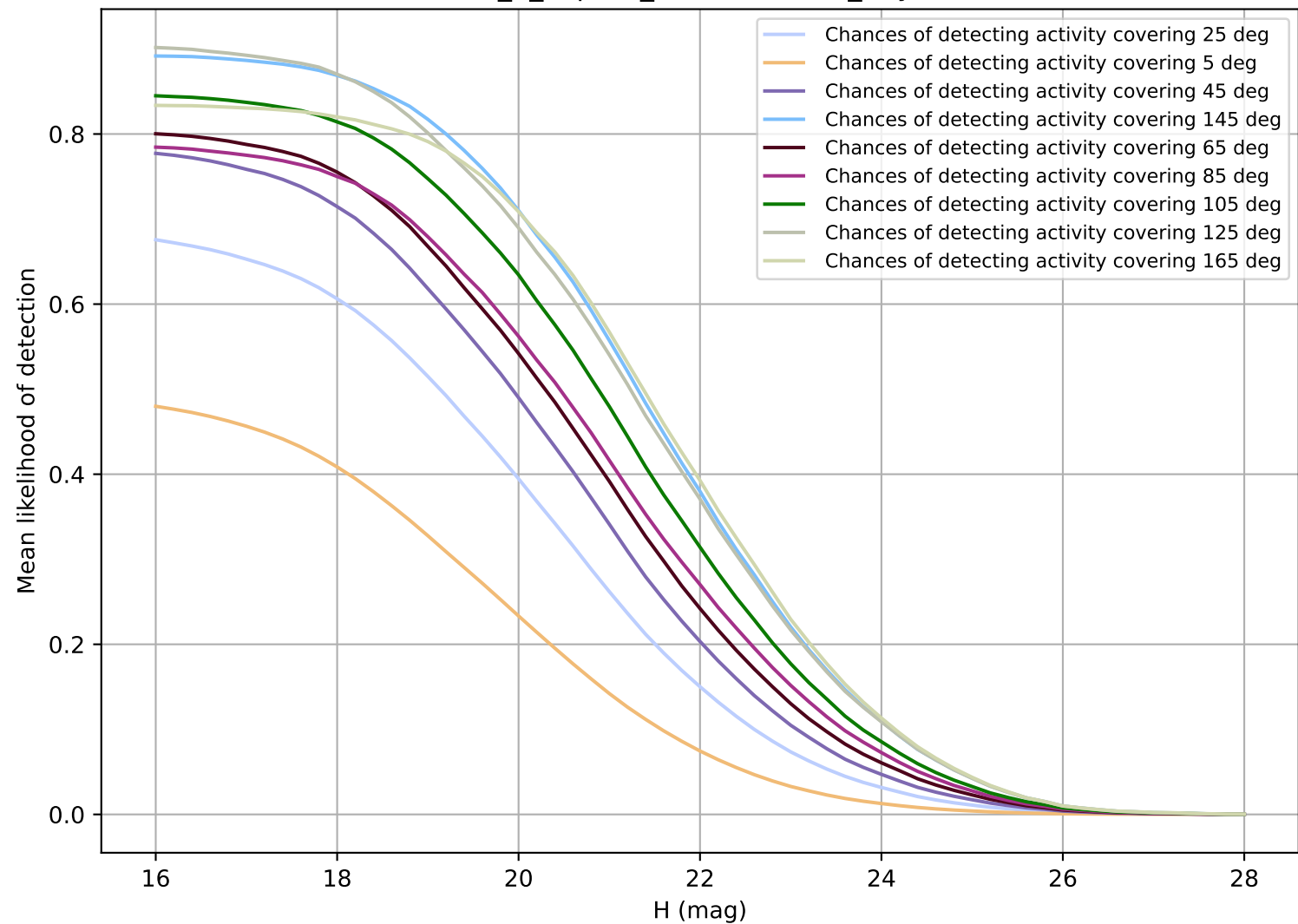
internal_u_expt60_nscale1.2v3.4_10yrs NEO
