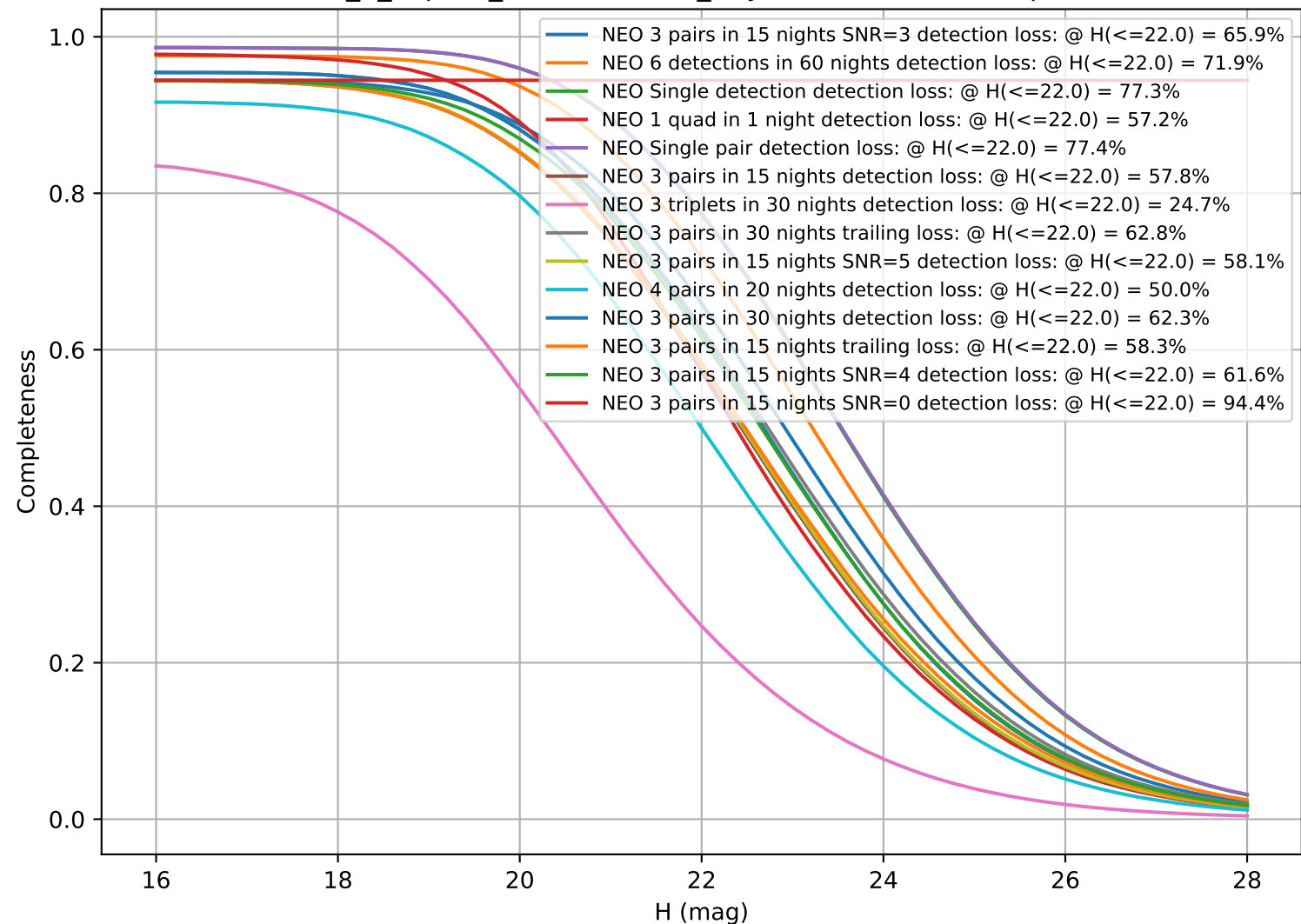
internal_u_expt60_nscale1.2v3.4_10yrs: CumulativeCompleteness
