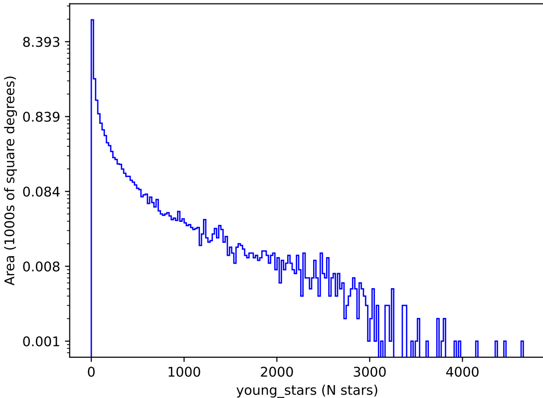
internal_u_expt60_nscale1.2v3.4_10yrs : young_stars
